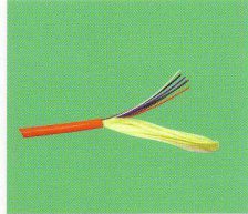
4 / 6 / 12 Core Multimode 62.5/125µm Tight Buffer
