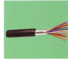
MK-FOUR 10 Pairs Outdoor Tel. Cable 0.63mm BC / Jelly Filled / 500M / Reel P/N: MK4-10500JB
