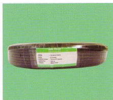
MK-FOUR 2 Pairs + 2 Core Control Cable 6Cx7x0.2mm TC / 100M / Roll P/N: MK4-6101
