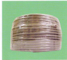
MK-FOUR 16 Pairs Telephone Cable 0.50mm BC / 100M / Roll P/N: MK4-16100
