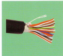
MK-FOUR 20 Pairs Outdoor Tel. Cable 0.63mm BC / Jelly Filled / 500M / Reel P/N: MK4-20500JB
