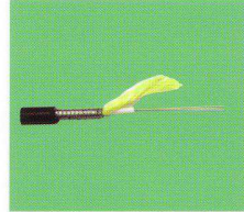
4 / 6 / 12 Core Singlemode & Multimode 62.5/125µm & 50/125µm Central Code Tube Design
