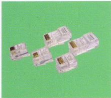
Modular Plugs RJ11 (4P4C), RJ11 (6P4C) RJ12 (6P6C), RJ45 (8P6C)
