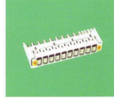
10 Pairs Magazine Loaded with 3 Pole Fail Safe Gas Tube Arrestor P/N: MK4 V11
