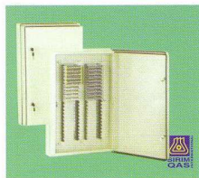
MK-FOUR Electro-Galvanized Metal Box 100, 200 & 400 Pairs P/N: MK-4100, MK-4200 & MK-4400
